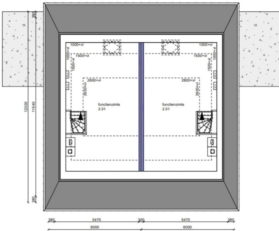
Zolder
